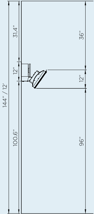
WALL MOUNT CLEARANCE
