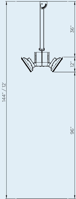
CEILING POLE CLEARANCE
