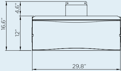
PRODUCT MEASUREMENTS 500 SERIES
